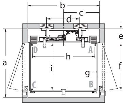
ABR - DCR OPPOSITE OPENING CODE 4
