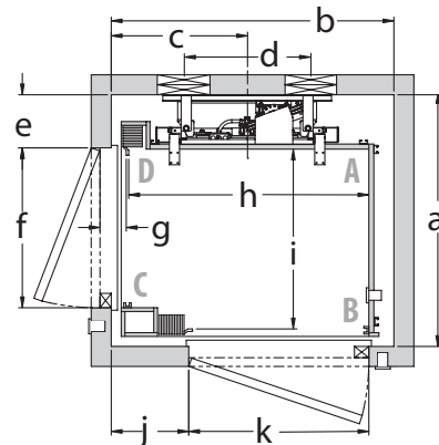
DCR-CB LEFT ADJACENT 90° OPENINGS CODE 6
