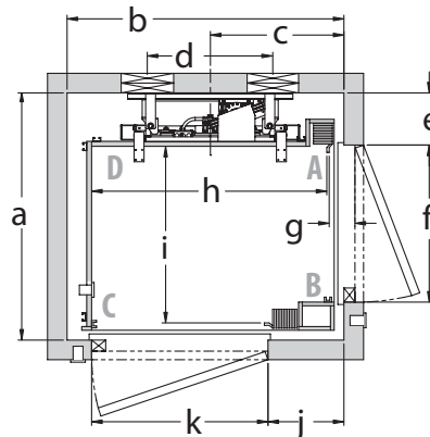
ABR BC RIGHT ADJACENT 90° OPENINGS CODE 5
